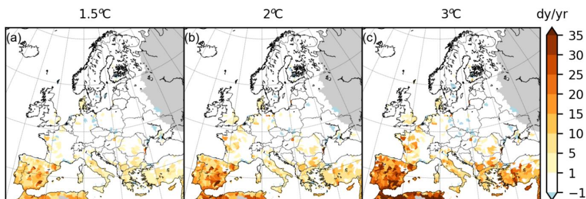
Figure 1. Projected change in water scarcity days ( WEI+ > 0.2 ) in a year compared with present day for a global temperature increase of (a) 1.5°C, (b) 2°C, and (c) 3°C. The results of both the 1.5°C and 2°C warming levels are based on the average of the 11 climate model simulations from both the RCP4.5 and RCP8.5 emission scenarios, while the results of the 3°C warming level are solely based on the 11 simulation of the RCP8.5 emission scenario.
