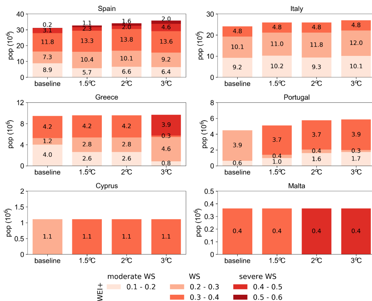
Figure A1. Projected number of people living in different gradations of water scarcity (WS) solely due to climate change for the baseline and under the different warming levels for the Mediterranean countries. Note that in Croatia no changes are observed and therefore Croatia is not presented.
